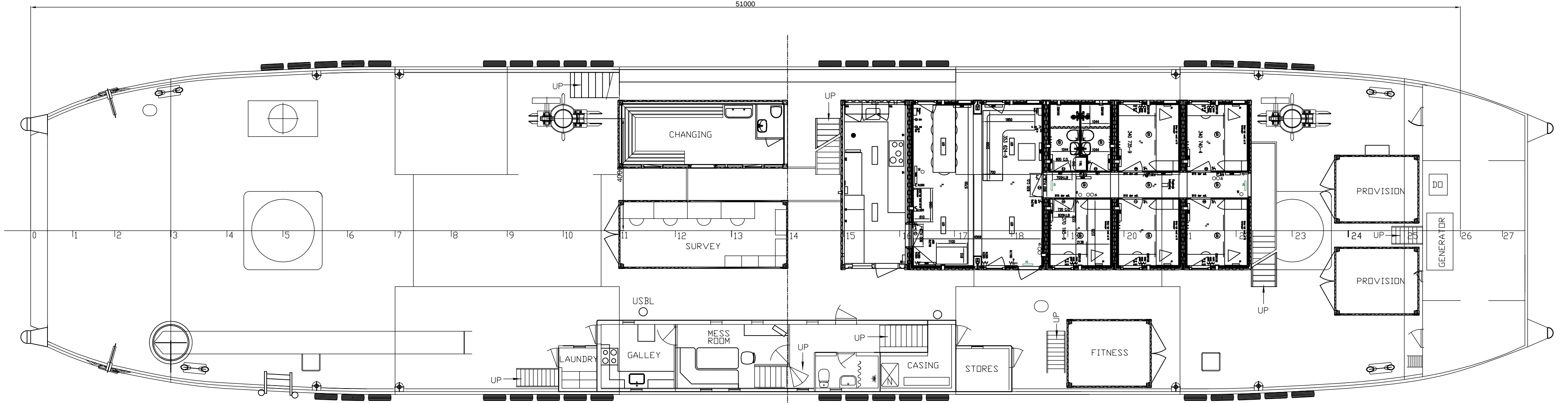
MAIN DECK
