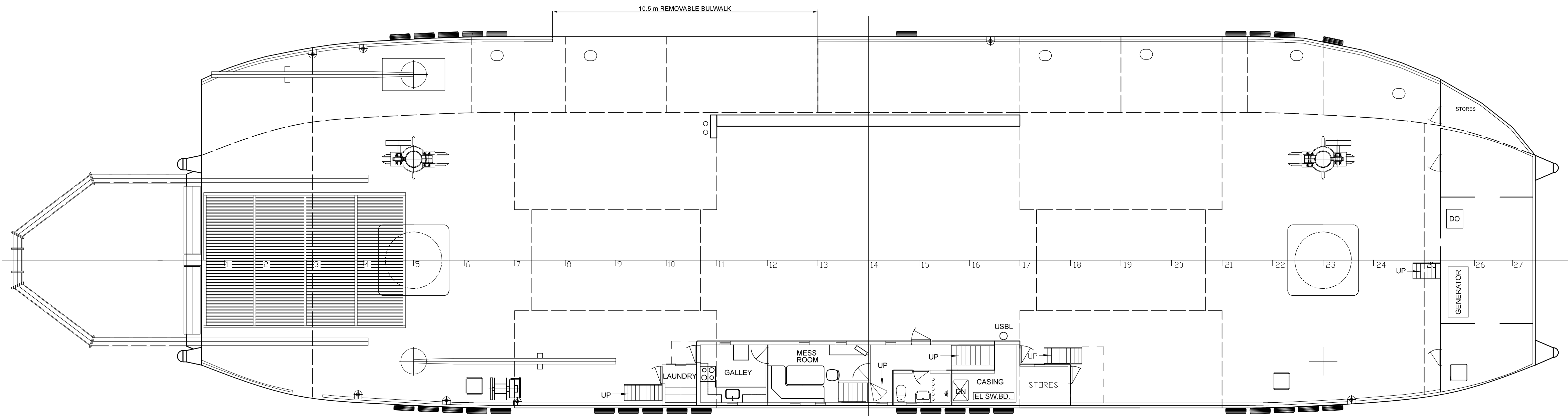
MAIN DECK
