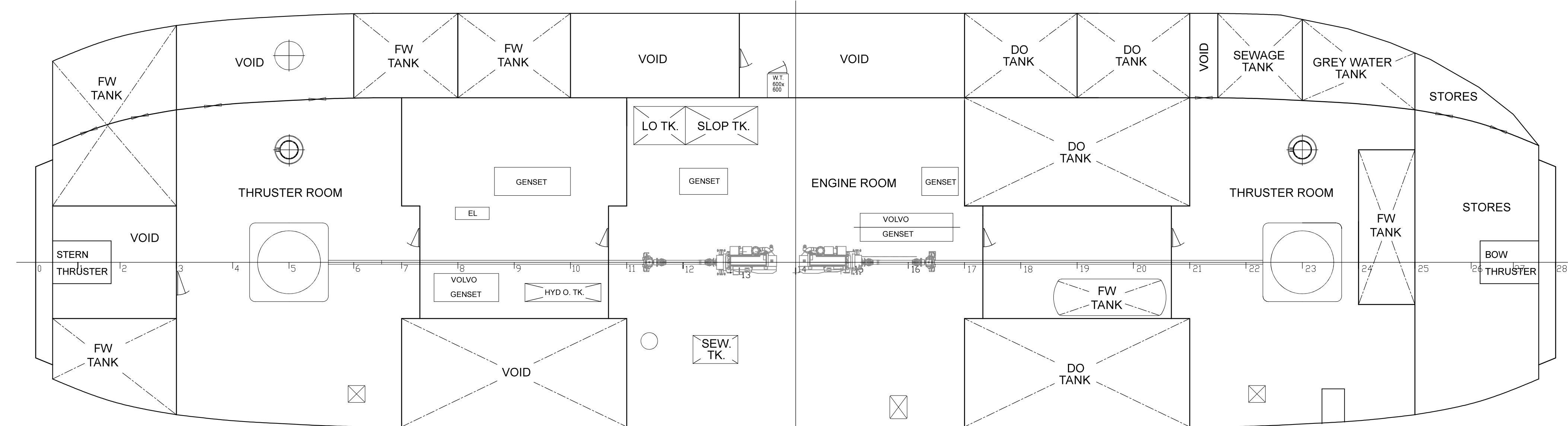
TANKTOP
